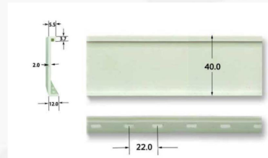
2. Rail fixed
